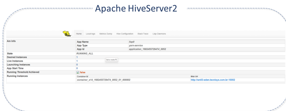
Figura 3 - Interface HiveServer2
