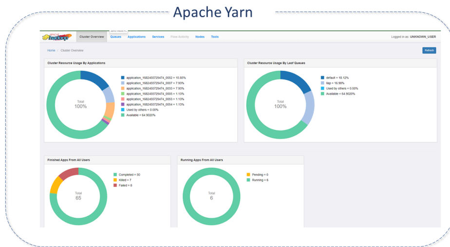
Interface YARN
