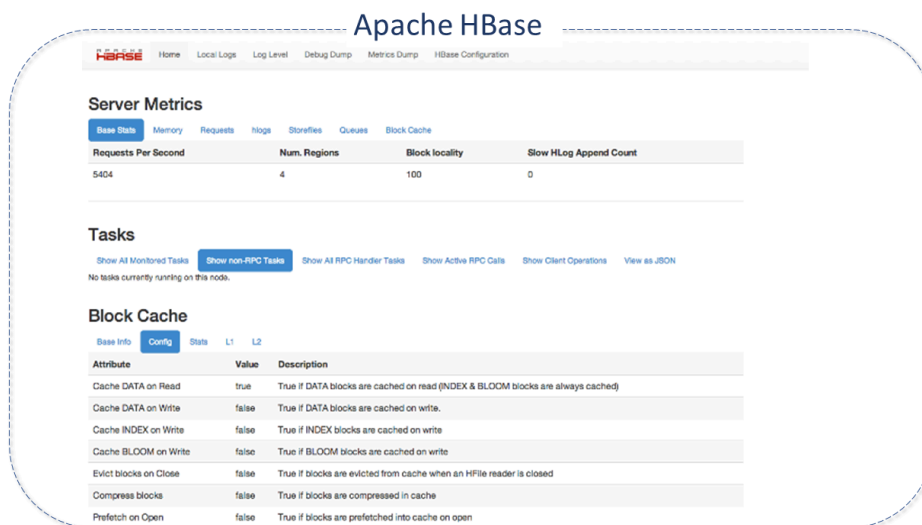
Figura 2 - Interface HBase
